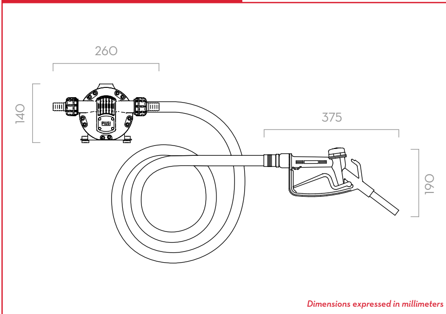
MANUAL NOZZLE
